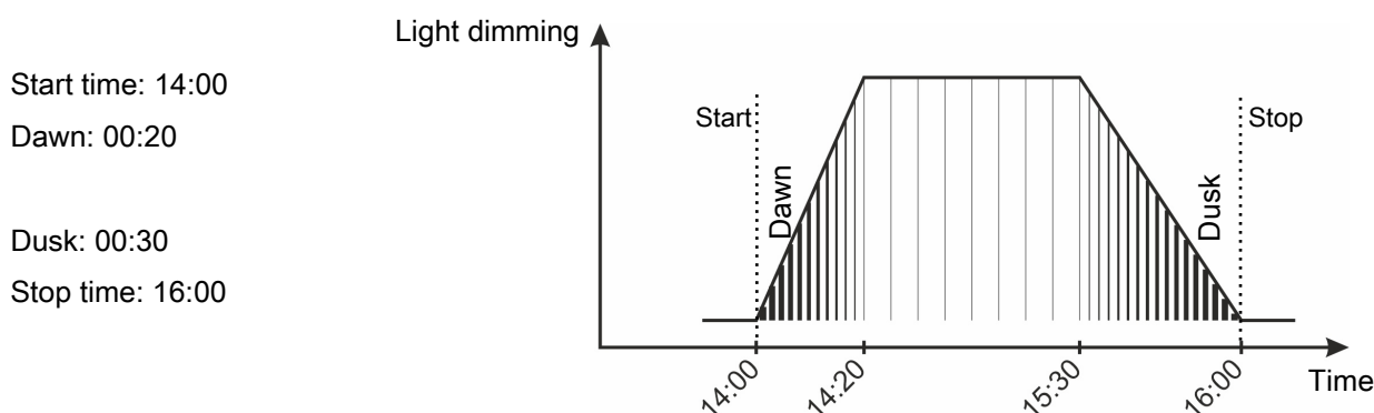
Figure 8: Normal light dimming Dawn and dusk are integrated in the light period.
