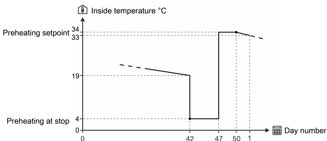
Figure 6: Example of setting of preheating.
